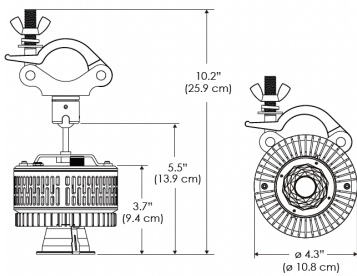
Mounting Bracket Dimensions ALL-CLP
