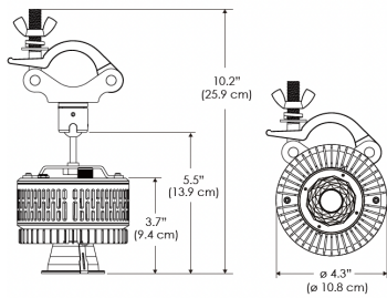
Mounting Bracket Dimensions ALL-CLP
