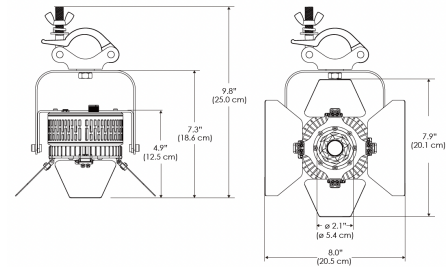
Mounting Bracket Dimensions ALL-CLP
